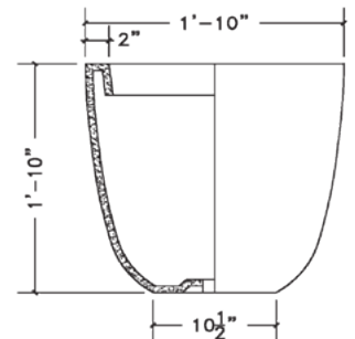
SPRING PLANTER 22" DIA X 22" H
