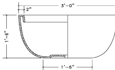
SPRING PLANTER 36" DIA X 22" H
