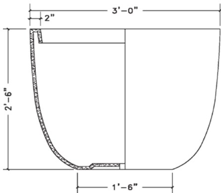
SPRING PLANTER 36" DIA X 30" H
